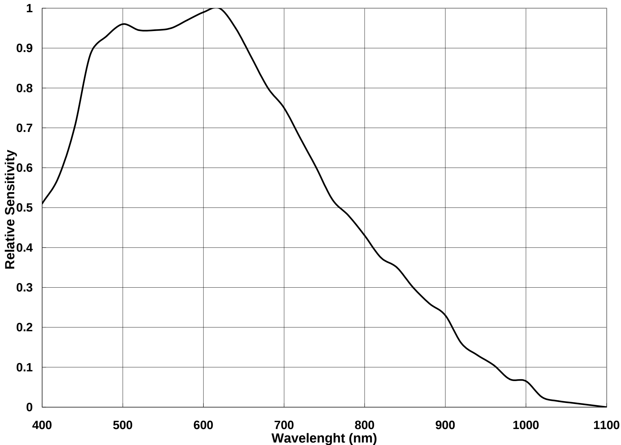
ICD-47 CCD Spectral Response
